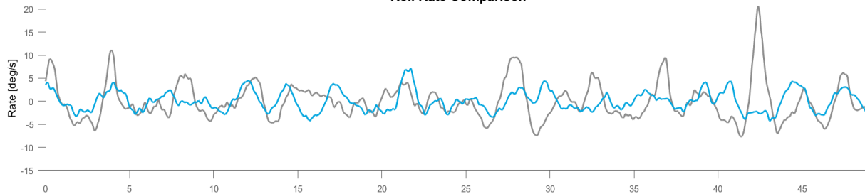
Bow Quartering Roll Rate Comparison
