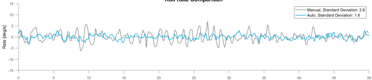
Stern Quartering Roll Rate Comparison
