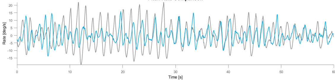
Pitch Rate Comparison
